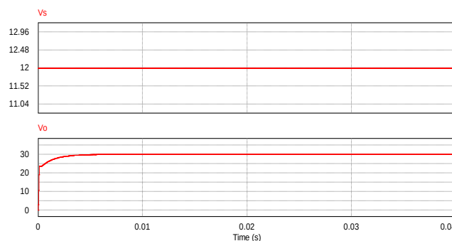
Figure 6. Input voltage wave form V_s and output voltage wave form V_o
