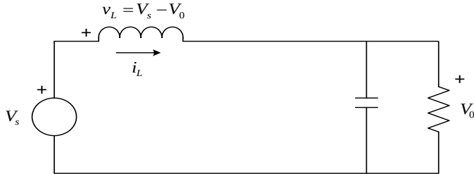
Figure 3. Equivalent circuit of DC-DC Boost converter when K open
