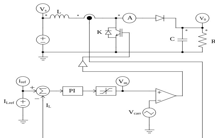
Figure 5. Control method based on inductor current
