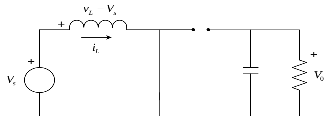
Figure 2. Equivalent circuit of DC-DC Boost converter when K closed
