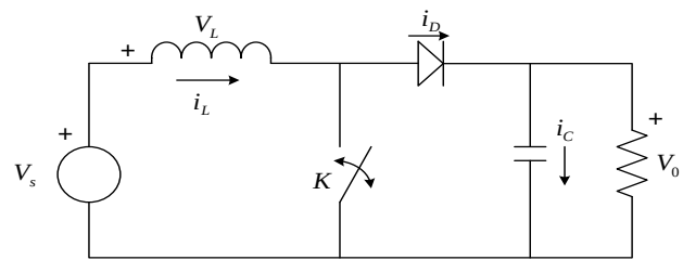
Figure 1. Topology of DC-DC Boost converter
