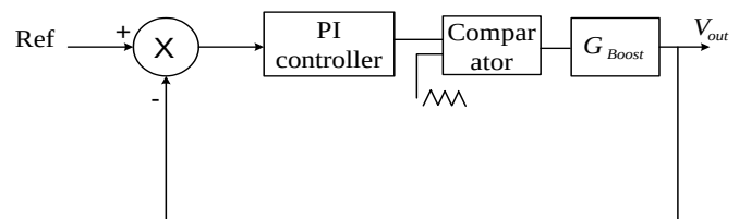
Figure 4. Control method scheme based on output voltage
