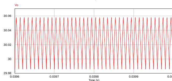
Figure 7. Output voltage ripple
